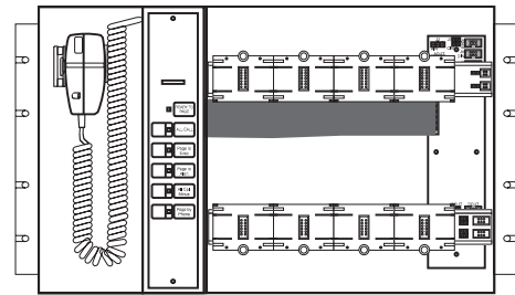
3-ASU/4 has Chassis, Audio Source Unit, Paging Common Control and rail space for four Local Rail Modules. Mounts in EST3 lobby enclosure.
